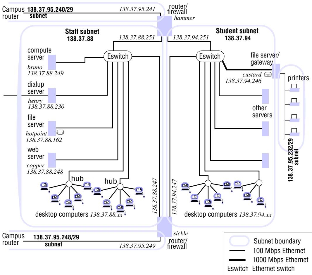
Figure 3.10 Simplified view of part of a university campus network
