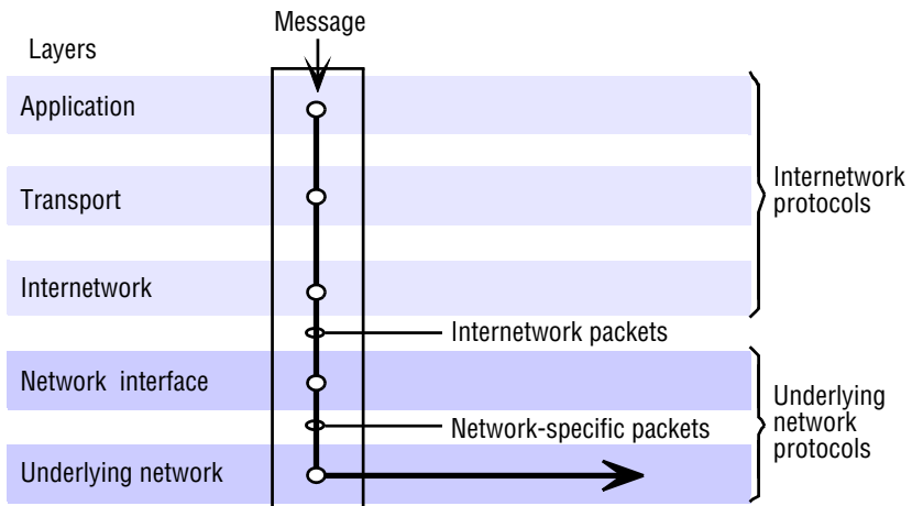
Figure 3.6 Internetwork layers
