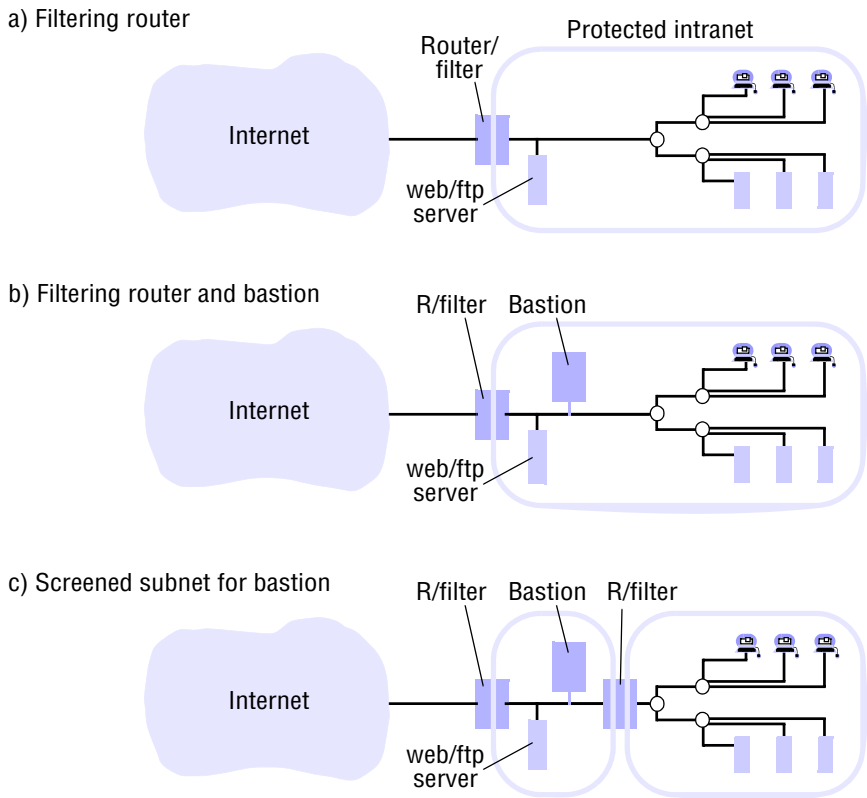
Figure 3.21 Firewall configurations
