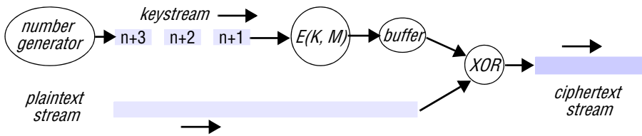
Figure 11.6 Stream cipher
