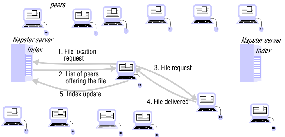
Figure 10.2 Napster: peer-to-peer file sharing with a centralized, replicated index
