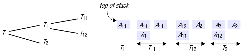
Figure 17.23 Nested transactions
