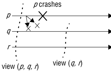
Figure 18.2 View-synchronous group communication
