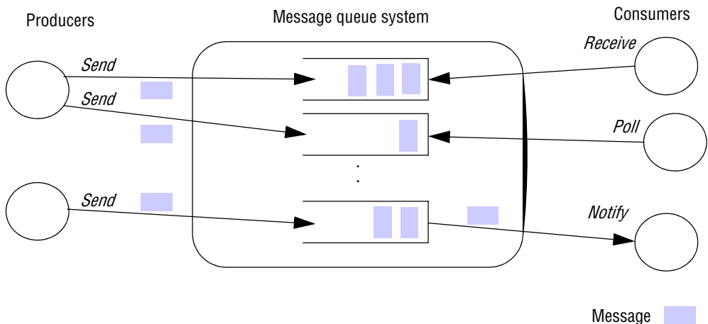
Figure 6.14 The message queue paradigm
