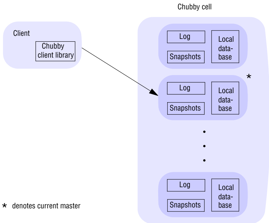
Figure 21.11 Overall architecture of Chubby
