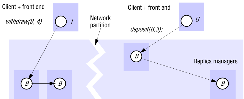
Figure 18.11 Network partition
