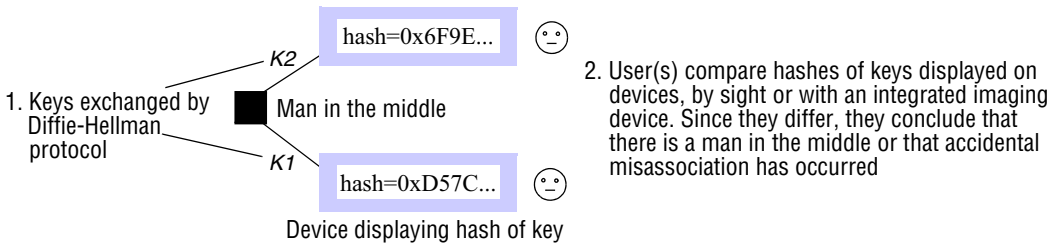
Figure 19.11 Detecting a man in the middle
