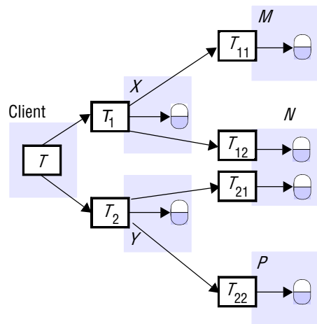
(b) Nested transactions
