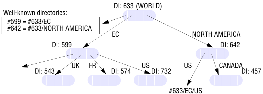
Figure 13.9 Restructuring the directory
