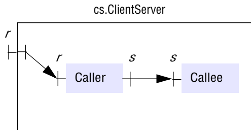
Figure 8.16 An example component configuration in Fractal
